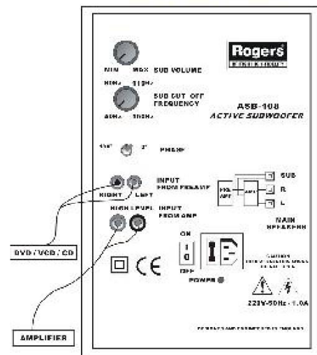
Rear Panel Diagram
